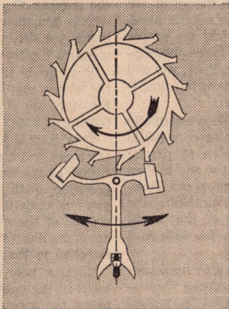
An escape wheel and oscillating pallet fork of a watch
